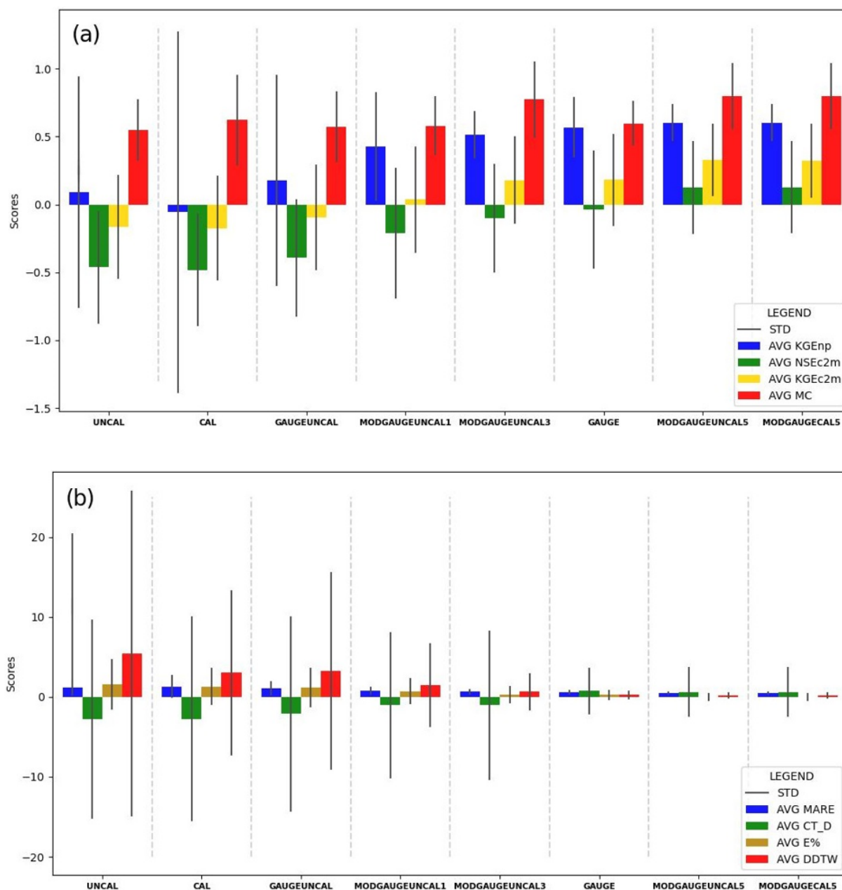
Figure 8. The histograms summarize the statistical analysis performed for the different scores, evaluating their average (AVG) and the standard deviation (SD). Panel (a) shows the quality scores (KGEp, NSEc2m, KGEc2m and MC), where the best performances are identified by a value equal to 1. In panel (b) (MARE, CT_D, E% and DDTW), the best performances are identified by values close to zero.
